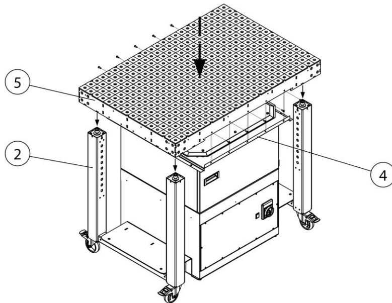
Fig. 24: Installation - Table top
