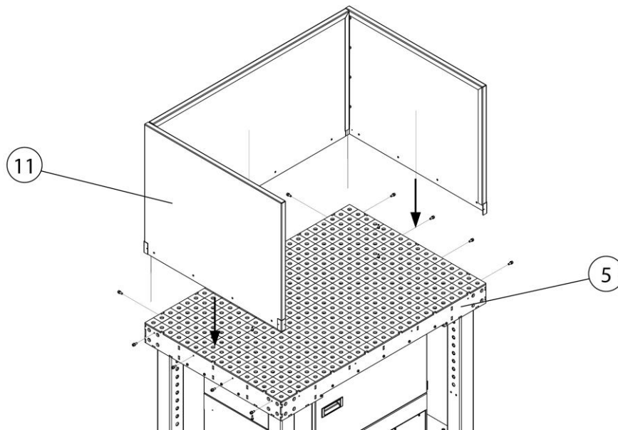
Fig. 26: Installation – side wall (optional)
