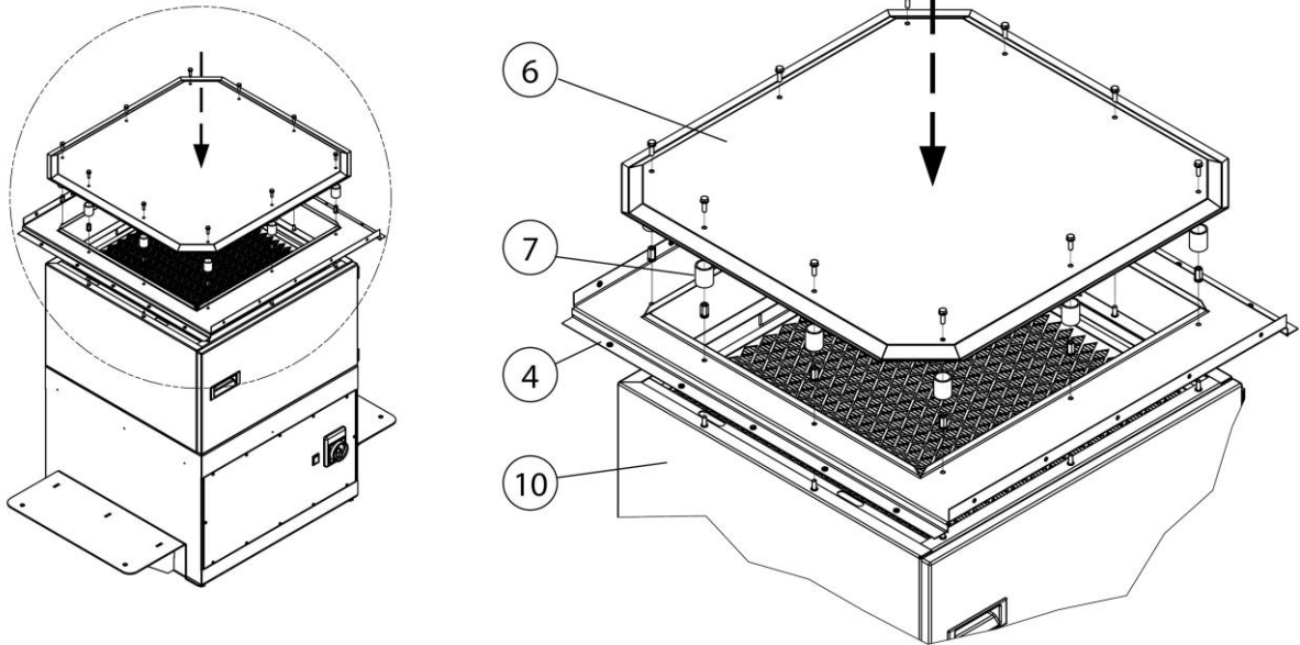
Fig. 22: Installation - Support frame + spark plate
