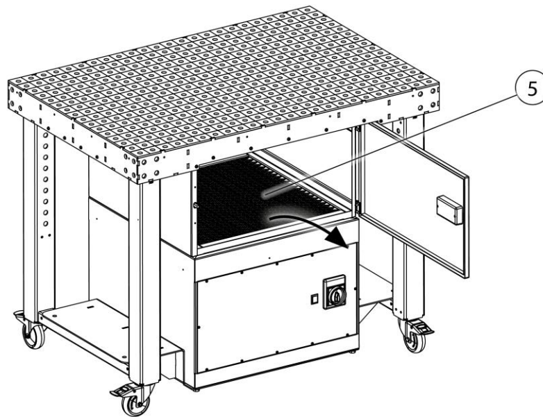
Fig. 31: Filter change – activated charcoal filter (optional)
