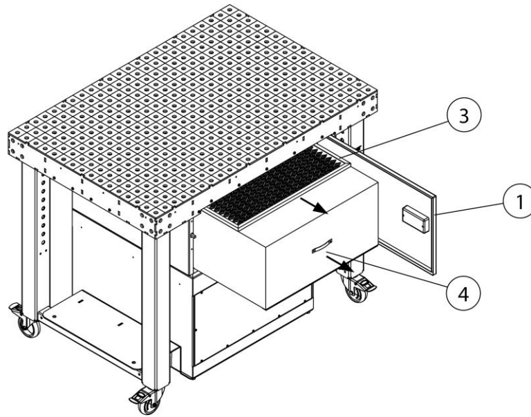
Fig. 30: Filter change – pre-filter + main filter
