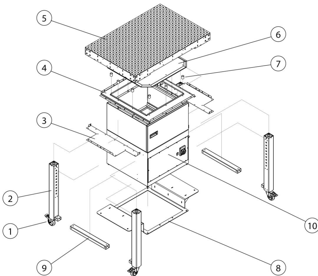
Fig. 19: Installation – Overview of components
