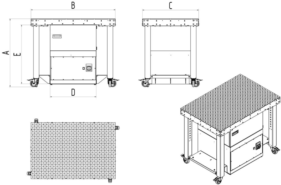
Fig. 33: Dimensions sheet
