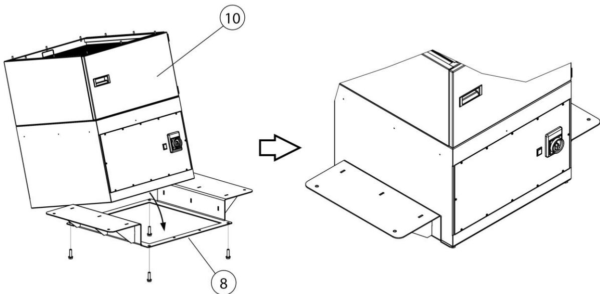
Fig. 21: Installation – Mount the filter unit on the support
