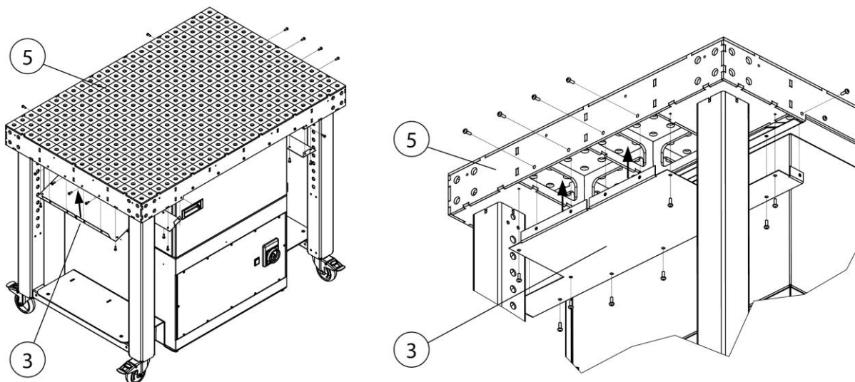
Fig. 25: Installation - Dust pan
