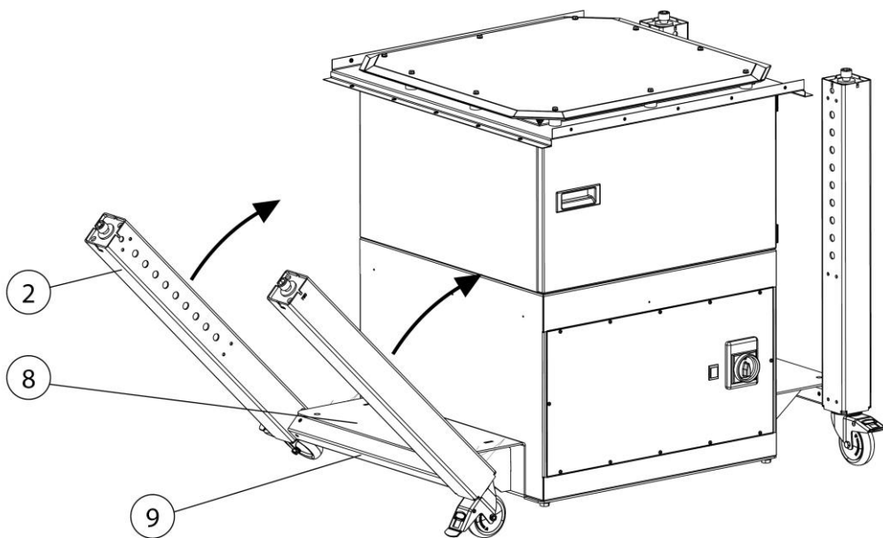
Fig. 23: Installation - Table legs
