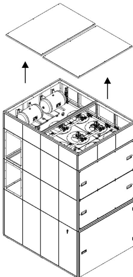
Fig. 239: Remover as chapas de cobertura
