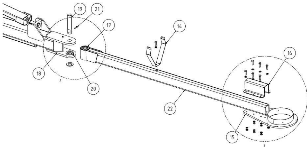
Fig. 31: Cantilever arm part 2
