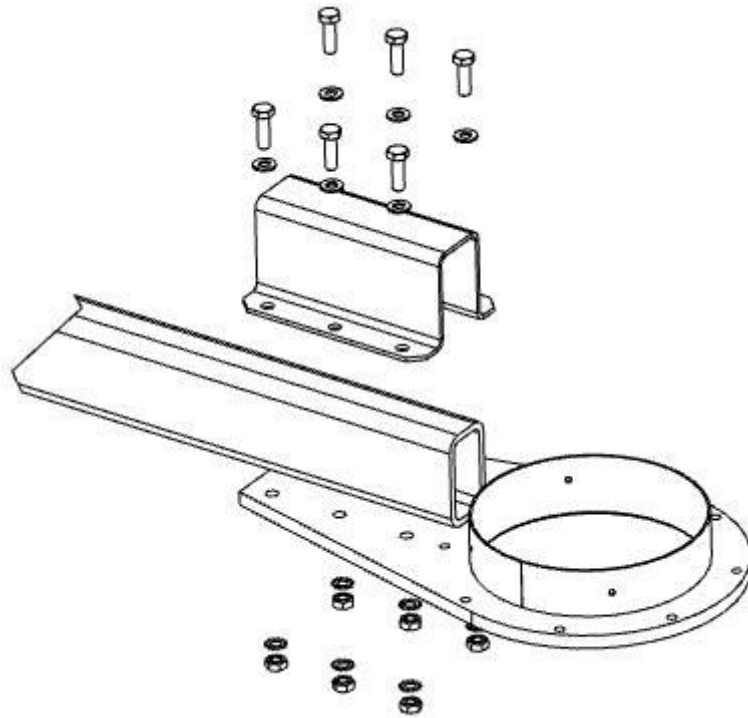
Fig. 32: Installing the extraction arm holder
