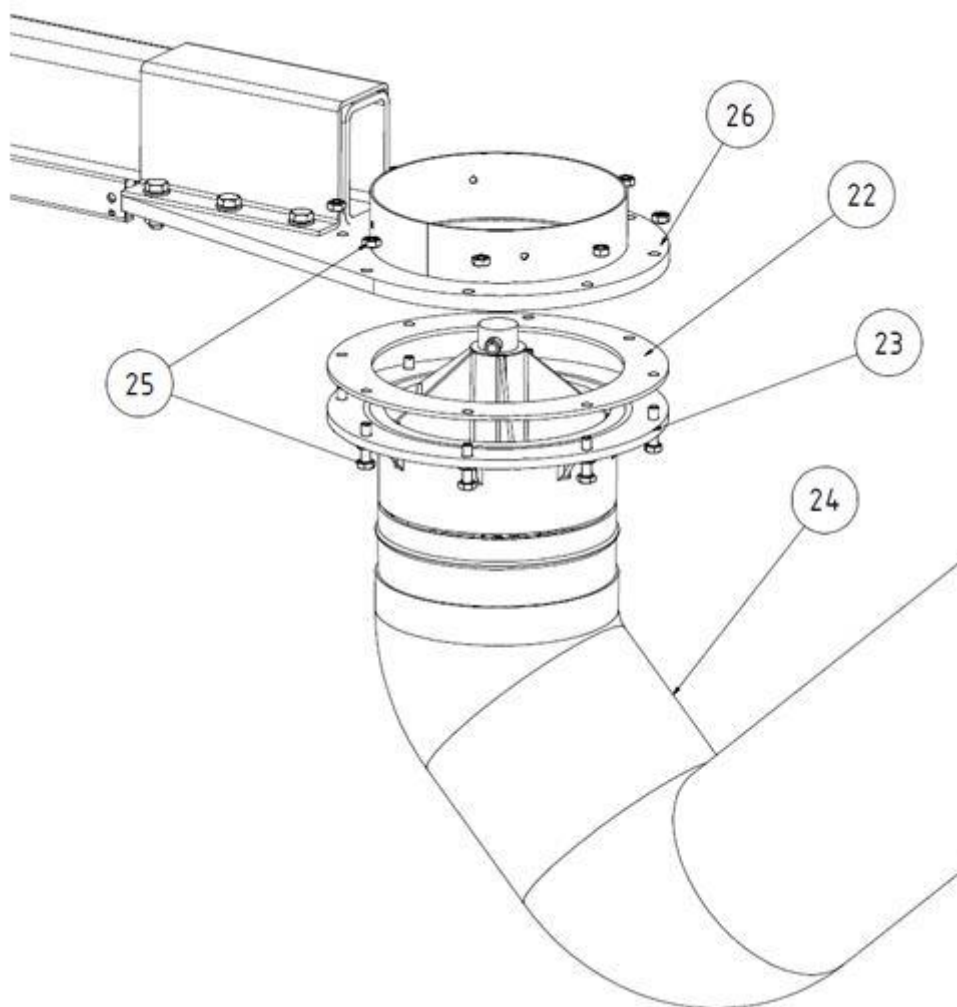
Fig. 34: Extraction arm on the cantilever arm
