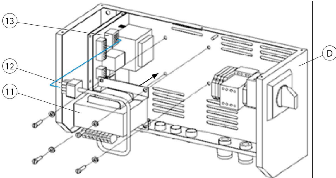
Fig. 40: Control Box - Retrofit Transformer
