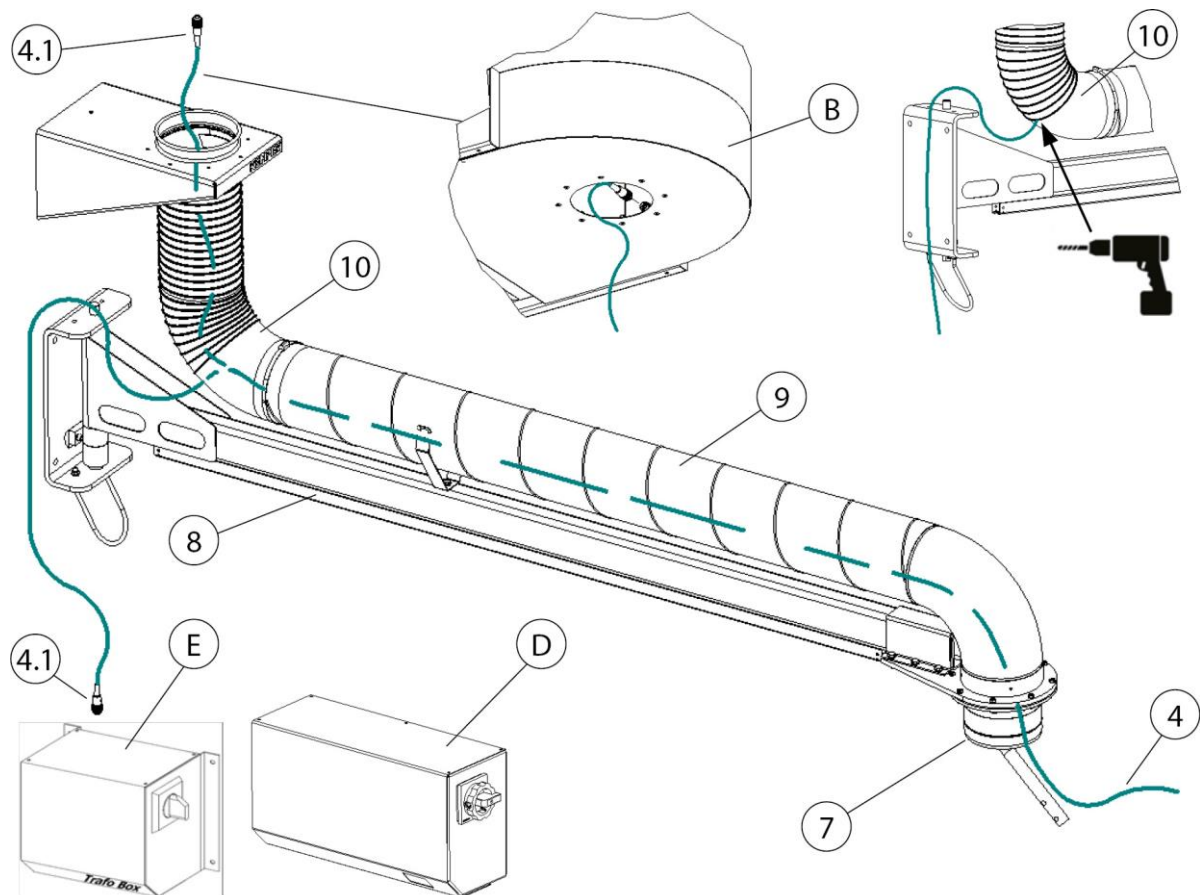
Fig. 39: Cable routing – extraction arms with crane cantilever
