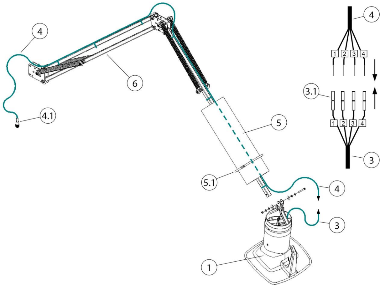
Fig. 42: Cable routing - extraction arm 2-4 metres
