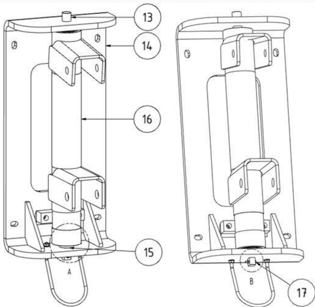
Fig. 28: Cantilever arm bracket
