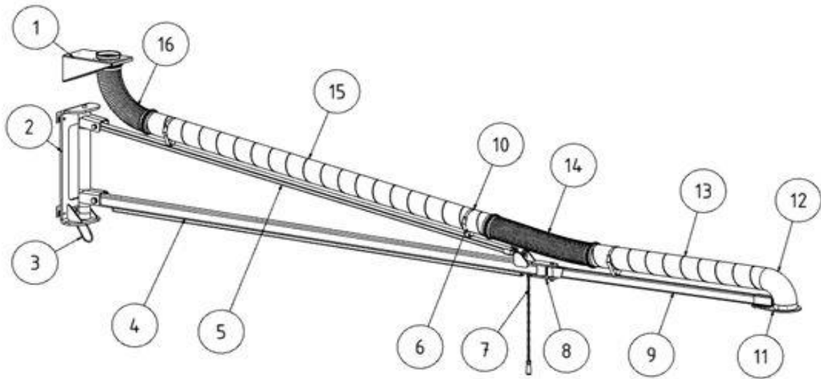
Fig. 24: Cantilever arm
