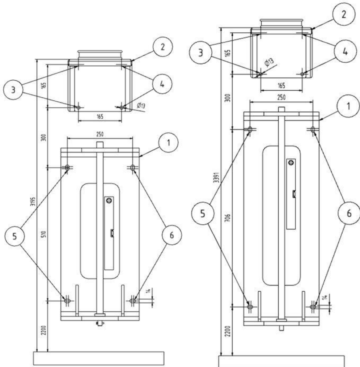
Fig. 27: Wall bracket
