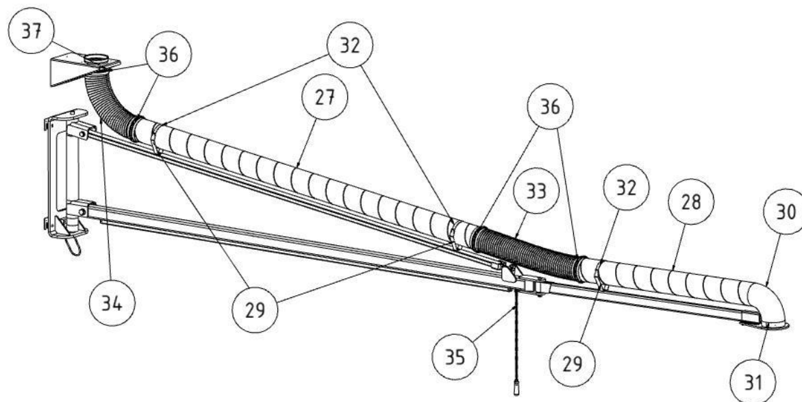
Fig. 36: Installing the spiral pipe
