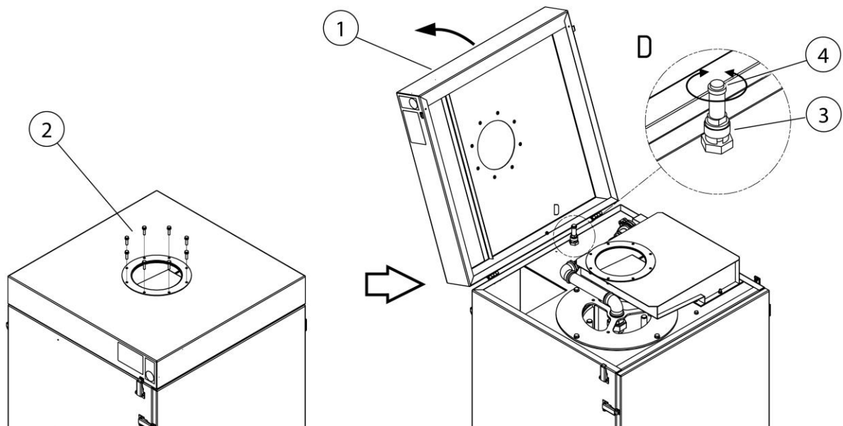
Fig. 11: Access to the compressed air safety valve
