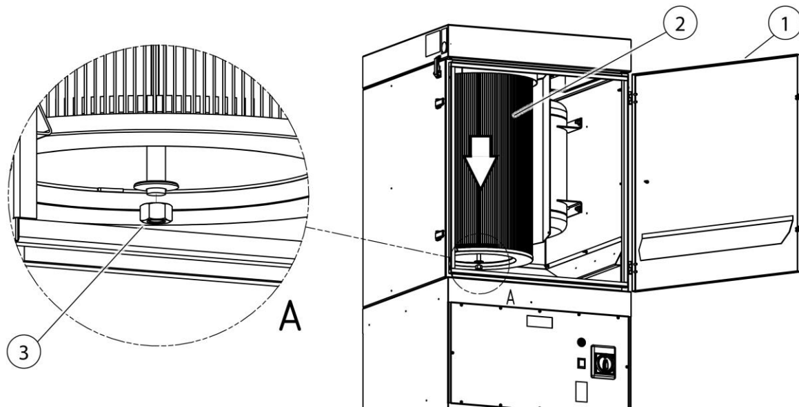
Fig. 8: Changing filters
