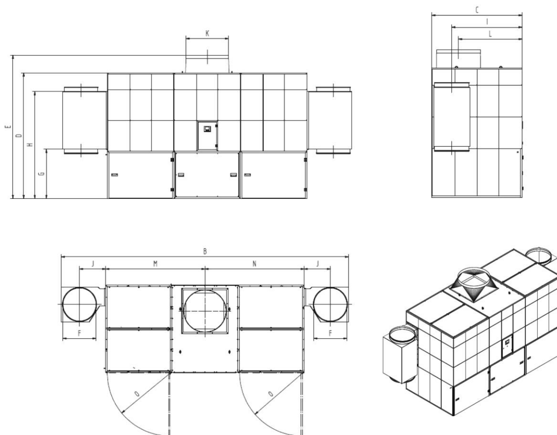
Sl. 360: List z merami 32160213 + 32160214 + 32180216 + 32180218
