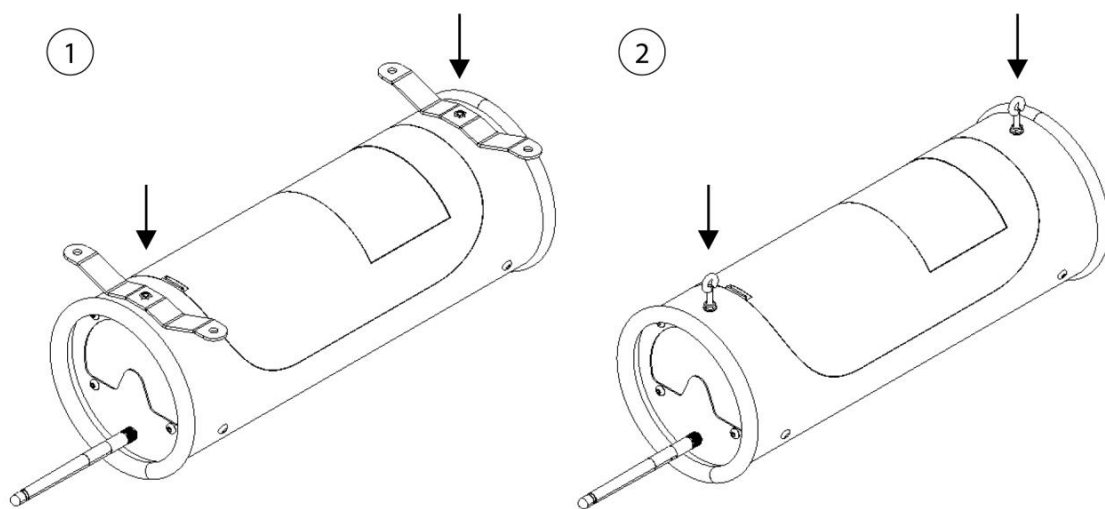
Abb. 7: Montage-Varianten
