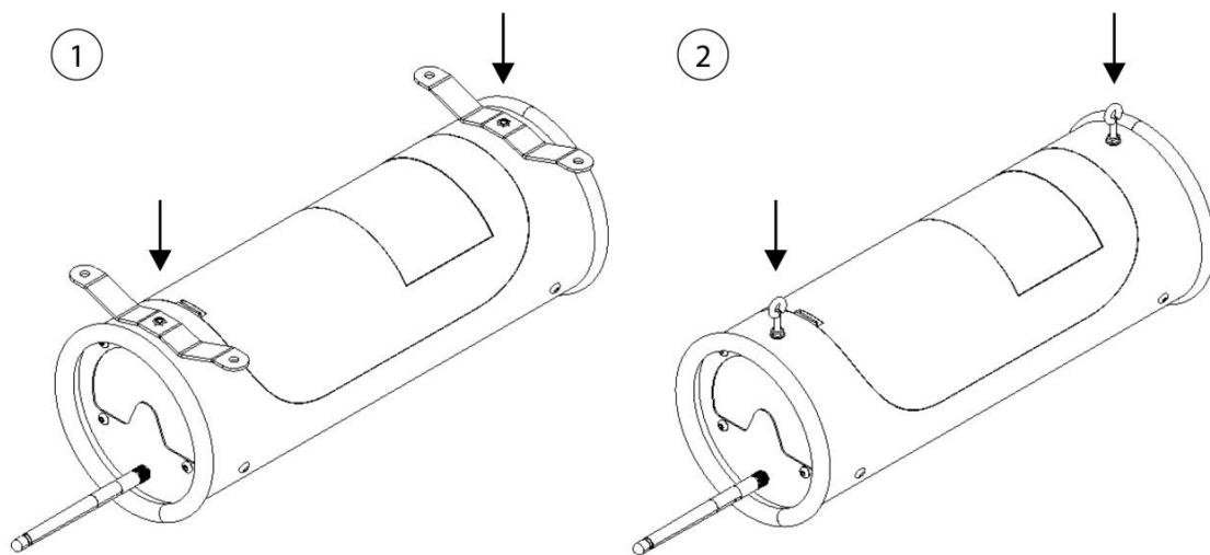
Fig. 20: Mounting variants
